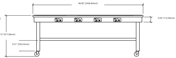
FRONT VIEW [96" Models]
