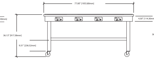
FRONT VIEW [76" Models]
